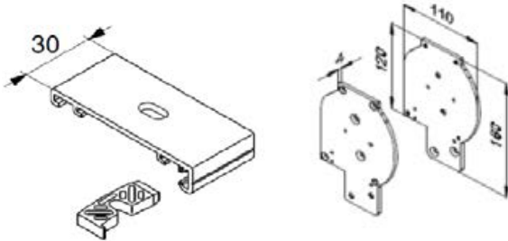
Bracket Detail
